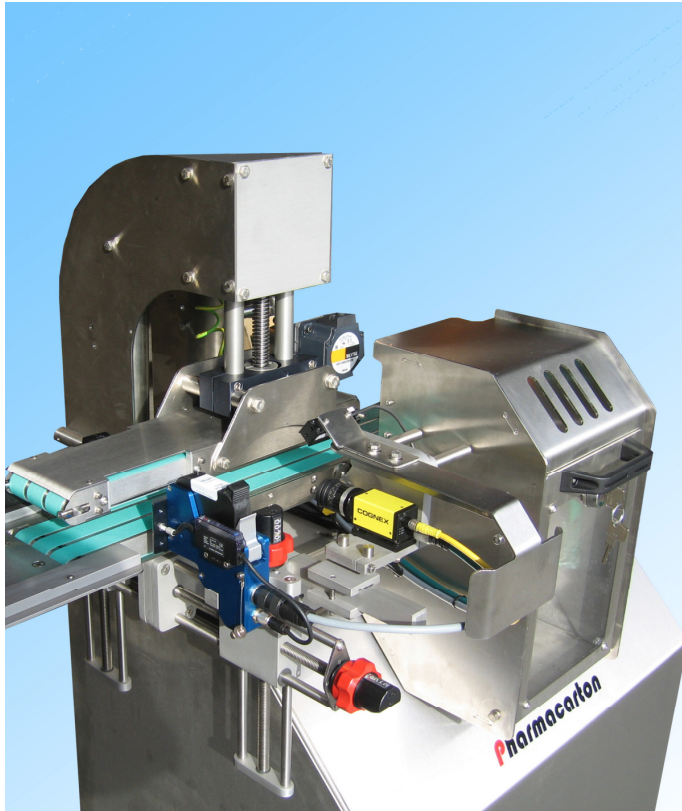
Pharmacarton Coding Station for Track & Trace and French CIP13
